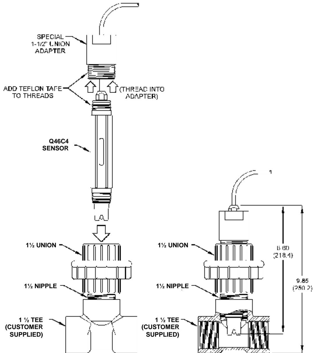
Figure 9 - 1.5" Union Mount
