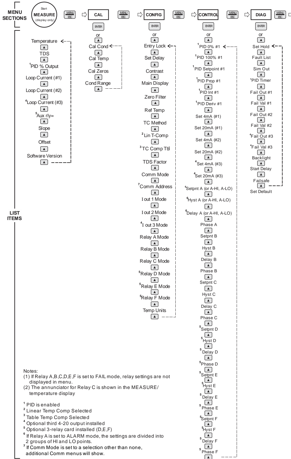
Figure 24 - Software Map
