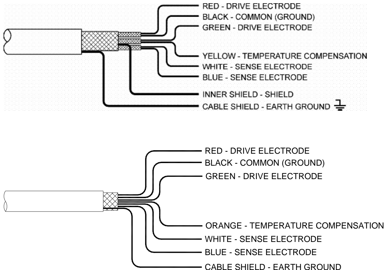
Figure 19 - Detachable Single Shielded Cable
