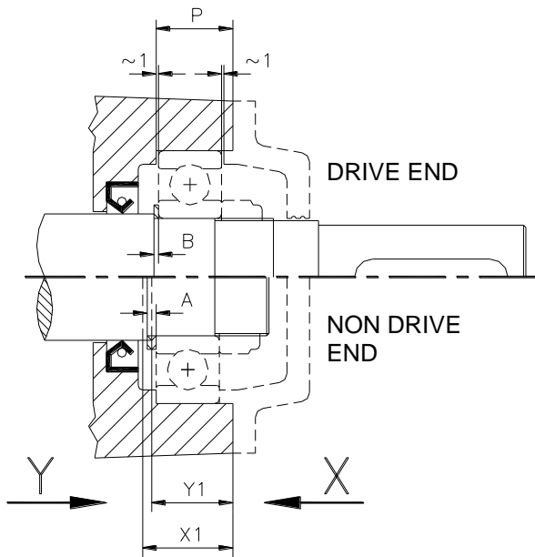
Fig. 9 "STANDARD" design
