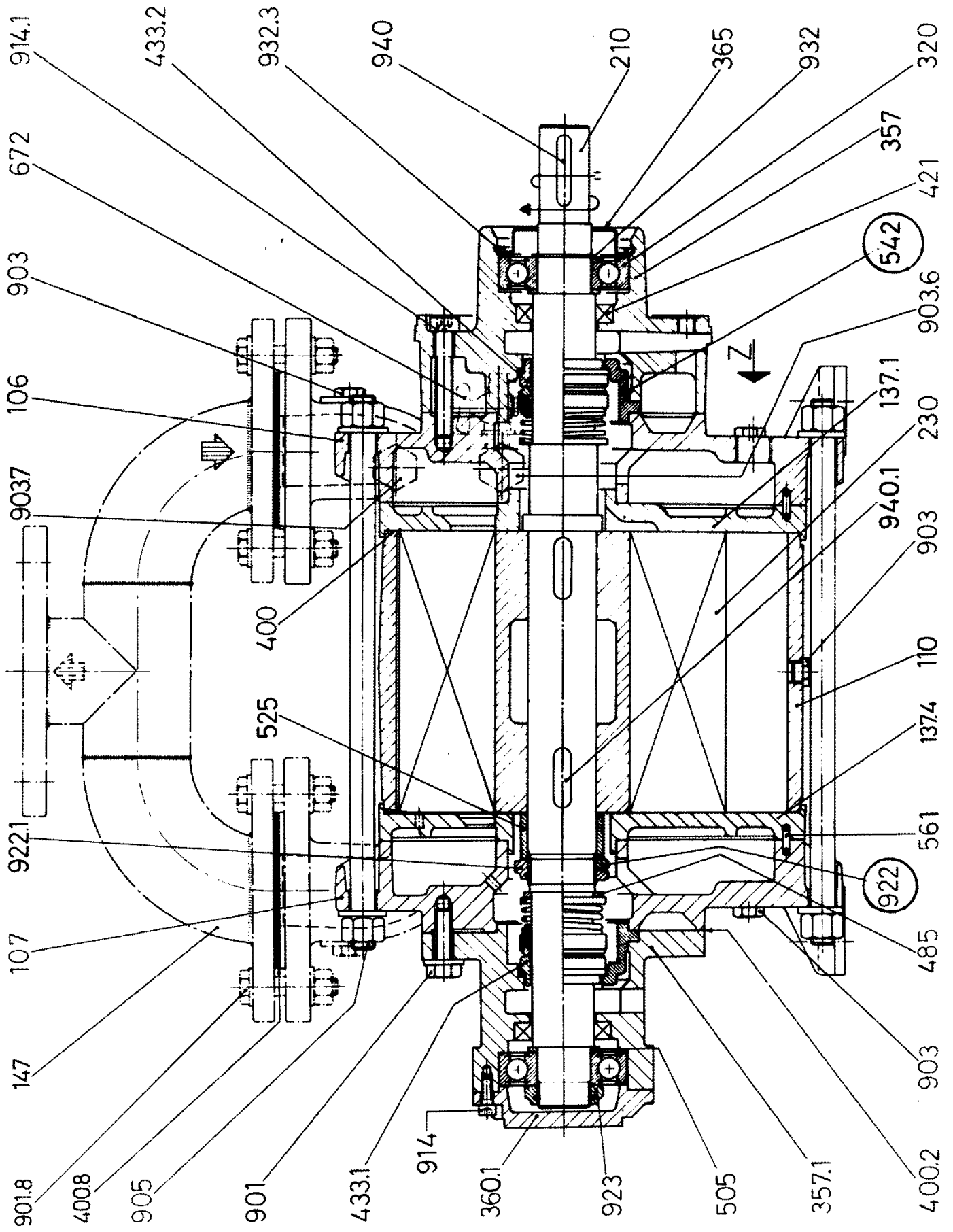
TRSC 40
