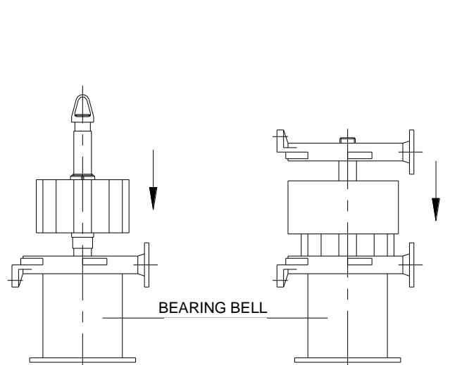
Fig. 30 and 31 - Pumps series TRS - TRV (step II & III)
