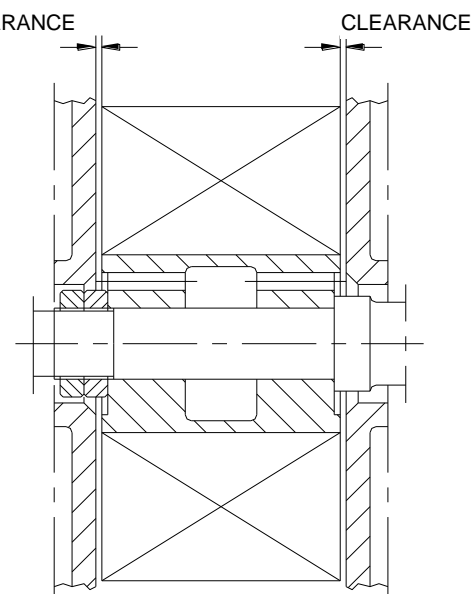
Fig.12 - Pumps series TRS - TRV
