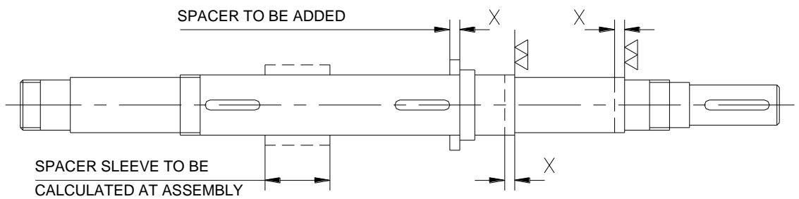
Fig. 21 Pumps series "TRH" (not for series 32 but applicable to TRHE 32-.../X)
