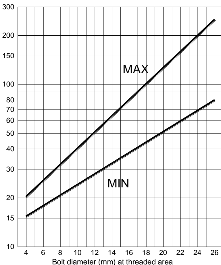
Fig. 34 TORQUE VALUES FOR VARIOUS BOLT SIZES
