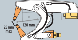
G11 8 bar/550 daN for TRAF0 PREMIUM PRO only 071766
