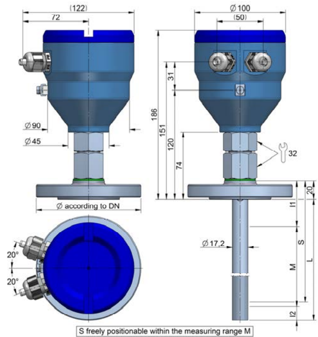
Coaxial probe, flanged connection
